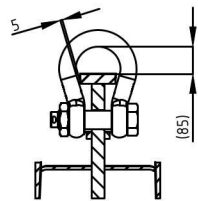
SECTION C-C SCALE 1 : 10
